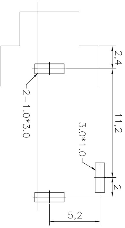
P.C.B. HOLE LAYOUT (BOTTOM VIEW)
